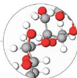
Pullulan
