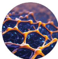
Chrysin Complex
