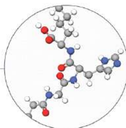
Palmitoyl Tripeptide -38
